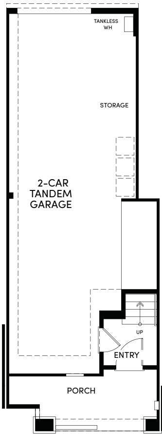
FIRST FLOOR
